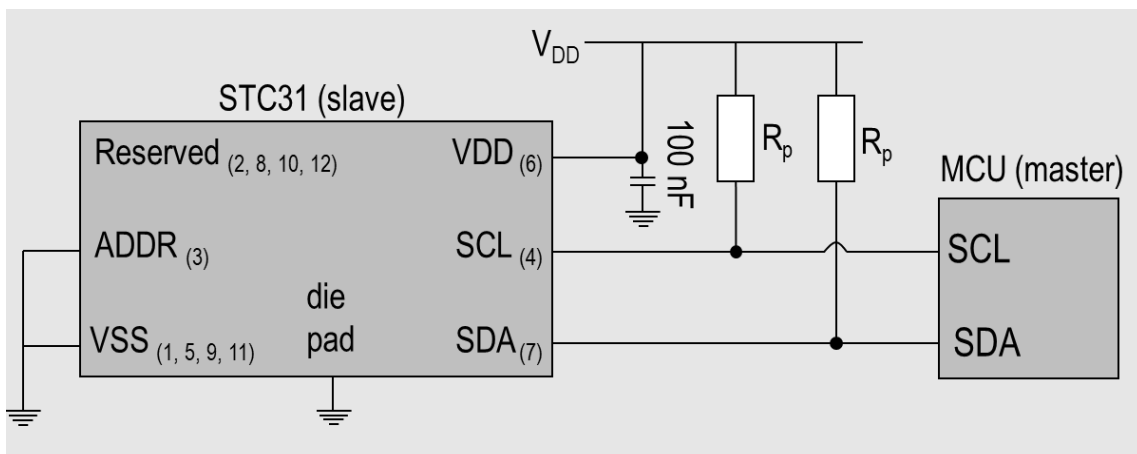
Figure 2: Typical application circuit. Please note that the positioning of the pins does not reflect the position on the reel sensor. This is shown in section 5. The pin numbers corresponding to the schematic in section 4.3 are indicated.
