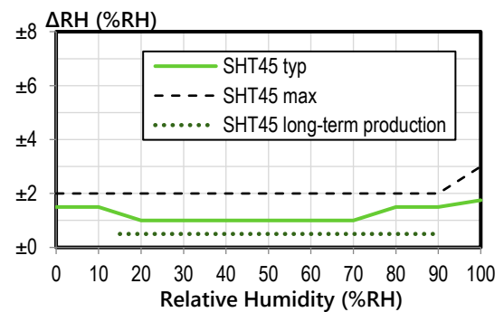
Figure 5. SHT45 typical, maximal and long-term production relative humidity accuracy at 25 °C.
