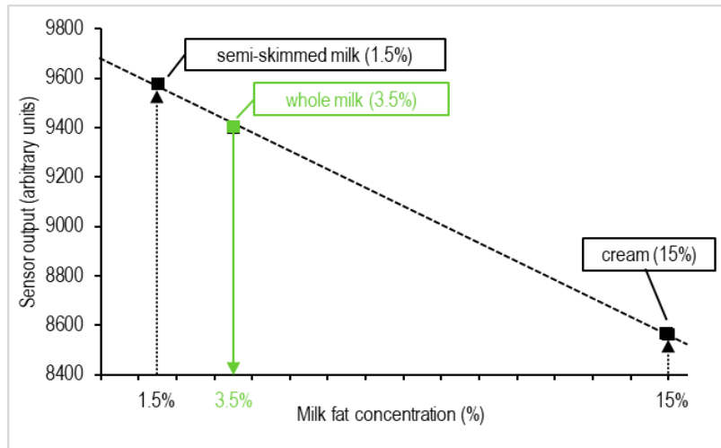
Figure 5. Sensor output vs. milk fat concentration. The dashed black line determined by measuring two anchor points (1.5% semi-skimmed milk and 15% cream, black squares) can be used to determine the fat concentration of other types of milk, e.g. 3.5% whole milk (green square).
