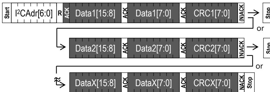
Figure 6. Schematics of I 2 C communication with SLF3x sensor. Dark areas with white text indicate that the sensor controls the SDA (Data) line. The I 2 C read sequences can be aborted with a NACK and STOP condition.
