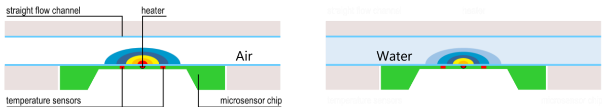
Figure 1. Thermal conductivity measurement at zero flow. Air has a low thermal conductivity, leading to a higher heater temperature (left), while water higher thermal conductivity leads to a lower heater temperature (right).
