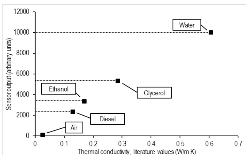
Figure 4. Thermal conductivity for selected fluids. Sensor output is in arbitrary units, while the literature values are in W/m K.
