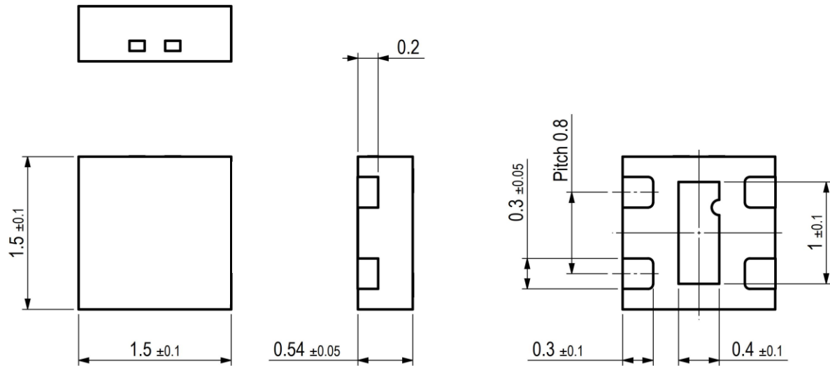
Figure 4. Dimensional drawing of the STS4x including package tolerances (units mm). The Pin 1 is identified by the cutout of the die pad, visible from the bottom.
