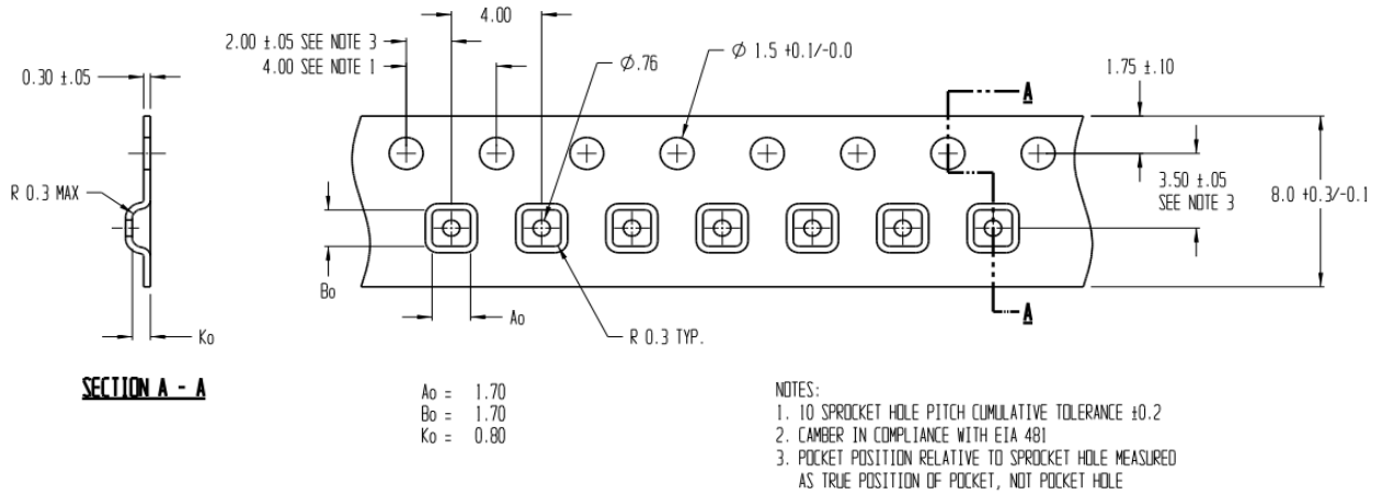
Figure 7. Tape and reel specifications including sensor orientation in pocket (see indication of two sensors on the right side of the tape).
