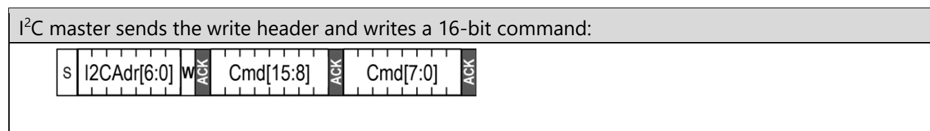
Figure 2: I 2 C sequences to send a command without an argument to the sensor.
