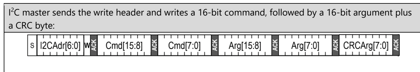
Figure 3: I 2 C sequences to send a command with an argument to the sensor.
