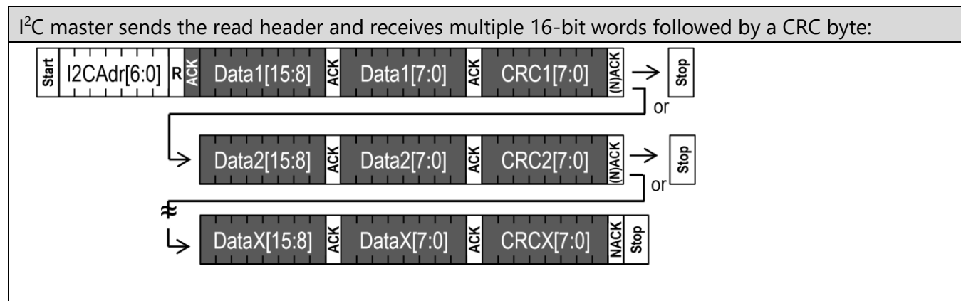
Figure 4: I 2 C sequences to read results from the sensor. Dark areas with white text indicate that the sensor controls the SDA (Data) line
