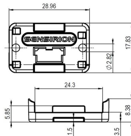
Figure 1: SDP800 Series cap. All dimensions in mm.
