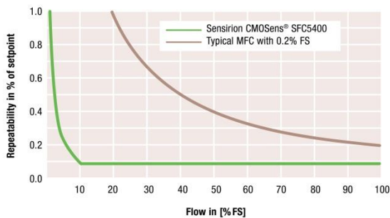
Figure 5: Repeatability comparison of the CMOSens® SFC54xx / SFM54xx device compared to a typical thermal mass flow controller / meter.
