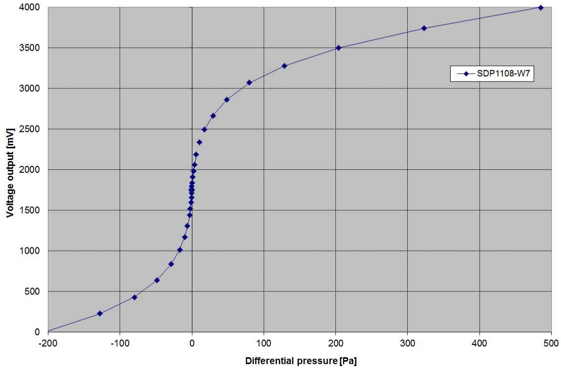
Sensoroutput SDP1108-W7
