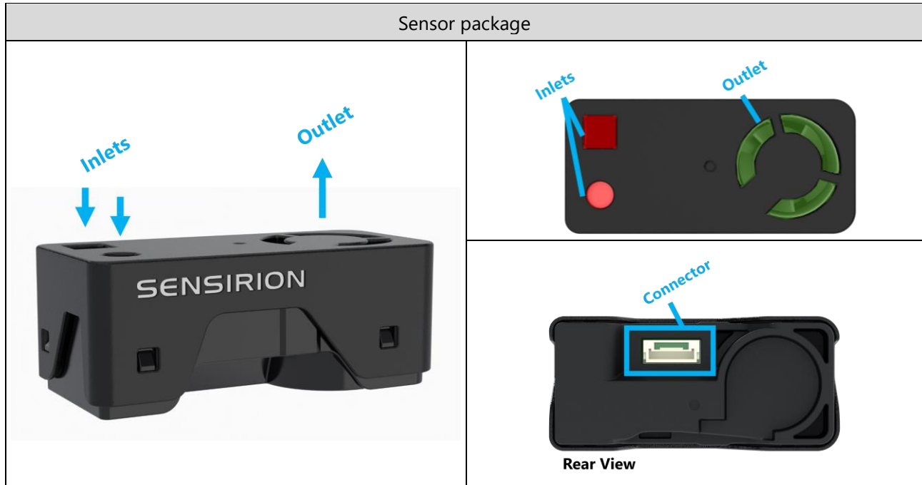
Figure 1. SEN6x package overview. Top right: Inlets (red, 56mm 2 ), outlet (green, 148 mm 2 )
