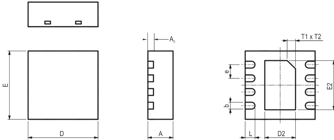
Figure 6. Dimensional drawing of STS32/33-DIS sensor package
