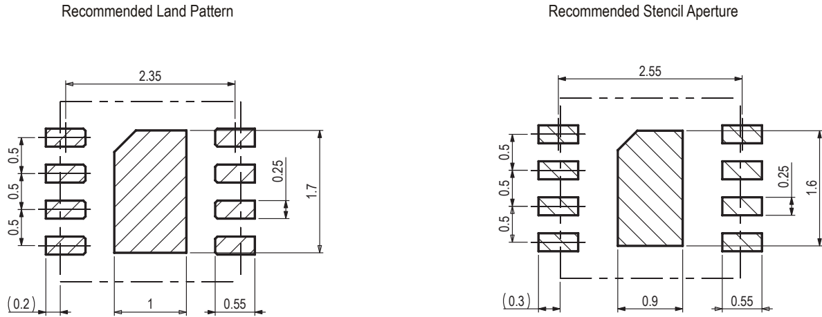
Figure 7. Recommended metal land pattern (left) and stencil apertures (right) for the STS32/33-DIS. The dashed lines represent the outer dimension of the DFN package. The PCB pads (left) and stencil apertures (right) are indicated through the shaded areas.
