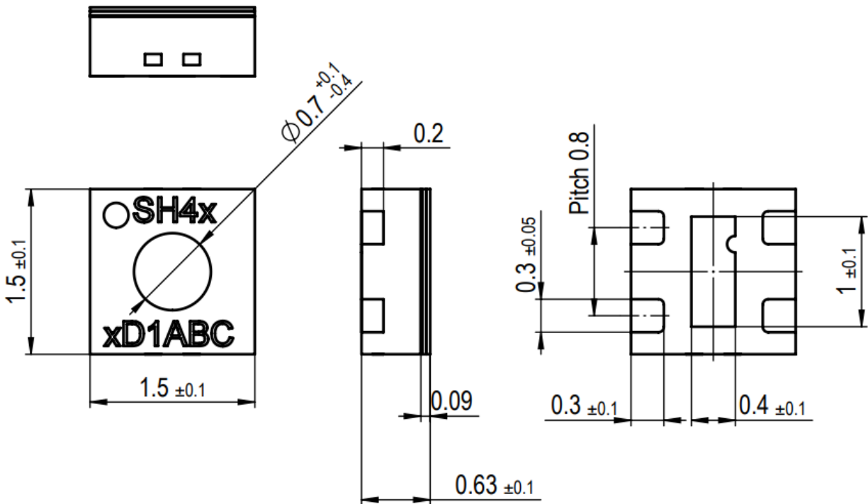
Figure 10. Dimensional drawing of SHT4xl-Digital with filter membrane including package tolerances (units mm).
