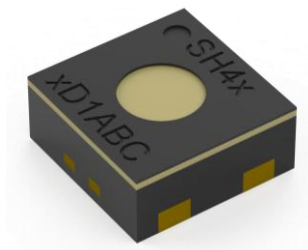
Figure 13. SHT4xl-Digital with integrated polyimide membrane, highlighting the beneficial flat geometry of the SHT4xl-Digital.
