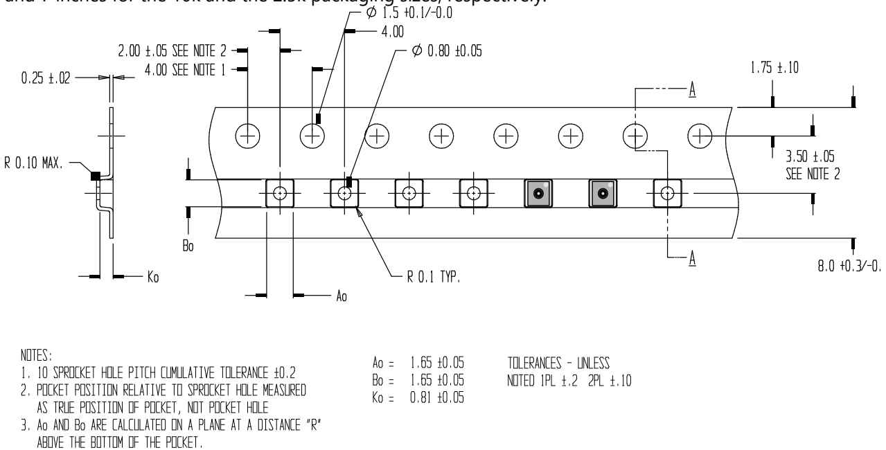
Figure 14. Tape and reel specifications including sensor orientation in pocket (see indication of two sensors on the right side of the tape).
