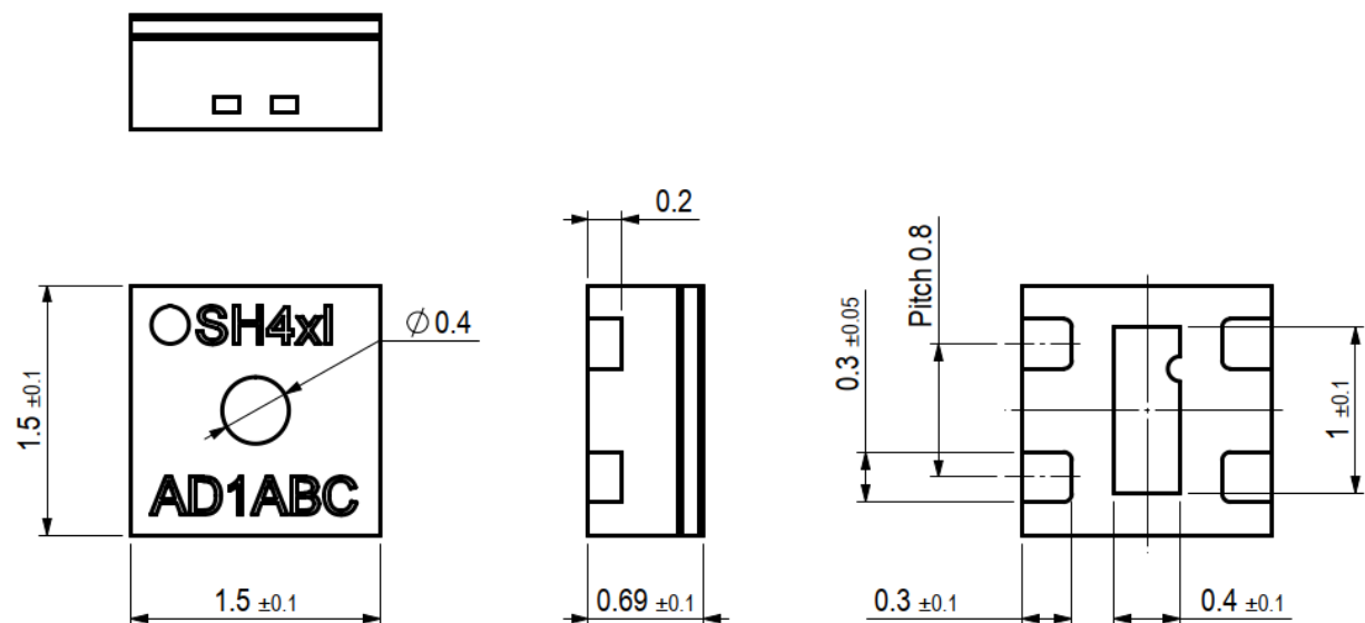
Figure 8. Dimensional drawing of SHT4xl-digital with filter membrane, including package tolerances (units mm)
