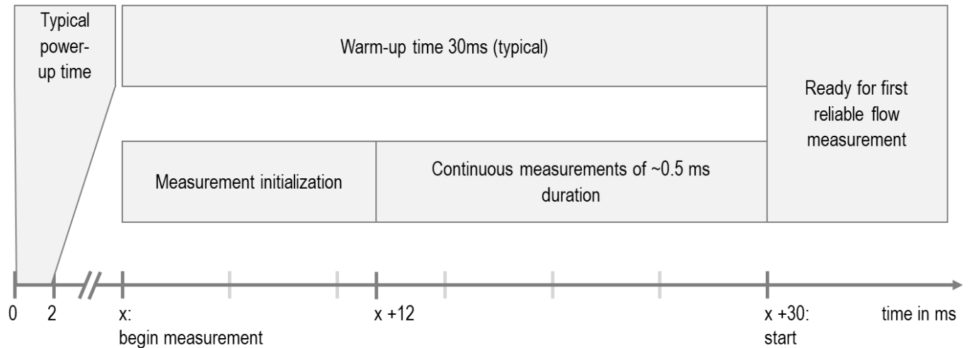
Figure 1: Time diagram upon start-up.
