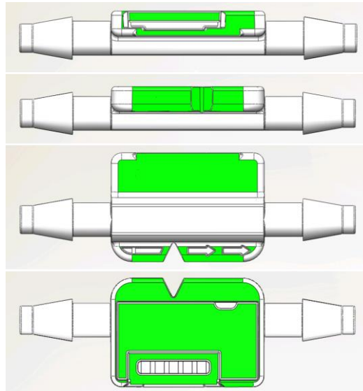
Figure 2: Surfaces (green) to be used to align and secure the LD20 sensor
