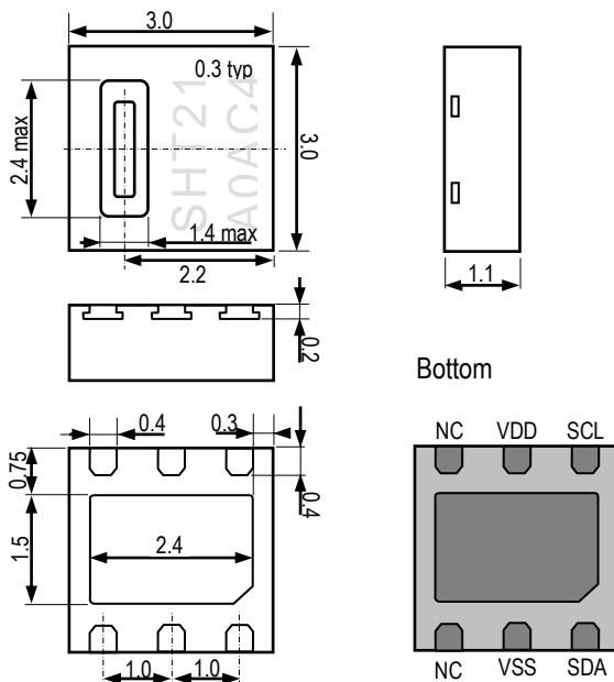
Figure 1: Drawing of SHT21A sensor package, dimensions are given in mm (1mm = 0.039inch), tolerances are \pm 0.1 mm. The die pad (center pad) is internally connected to VSS. The NC pads must be left floating. VSS = GND, SDA = DATA. Numbering of E/O pads starts at lower right corner (indicated by notch in die pad) and goes clockwise (compare Table 2).
